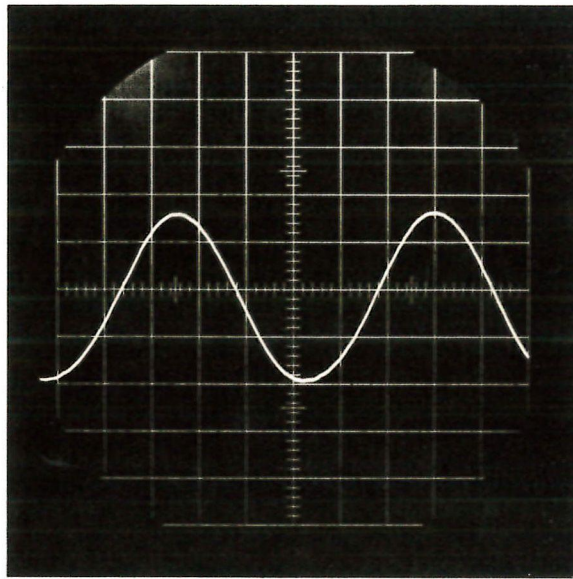
This unretouched photo shows the acoustic output of the system when driven by a 50-W sine wave signal at 35 Hz. A laboratory microphone was used to pick up the sound from the 4311. The signal from the microphone was connected directly to an oscilloscope and the trace photographed.
